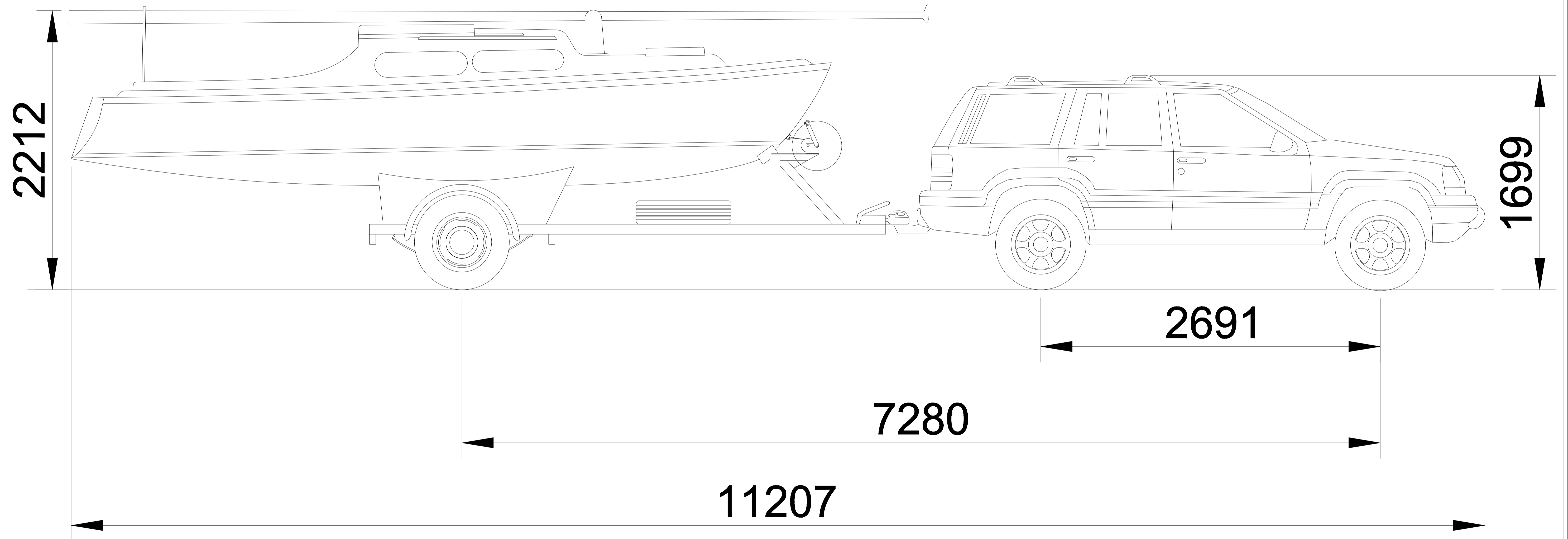
Towing Arrangement
